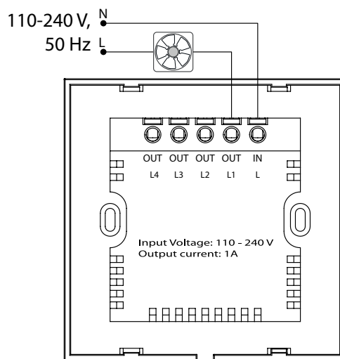
Wiring diagram (only for SGS E1)
