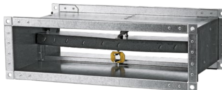
BSK1...72S normally open fire-resisting duct damper with mechanical drive mechanism.
