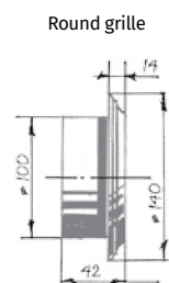
Round grille
