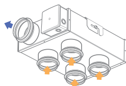
4 inlet pipes \varnothing 80 or 100 mm
