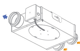
2 inlet pipes \varnothing 80 or 100 mm
