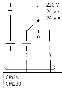
3 point controlling
