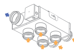
6 inlet pipes \varnothing 80 or 100 mm
