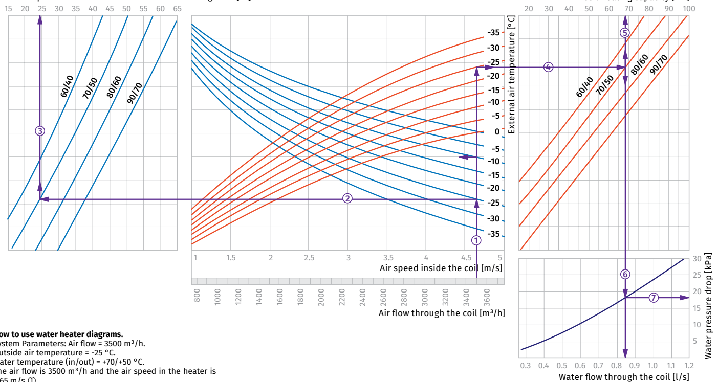
Air temperature downstream of the water heating coils [°C]
