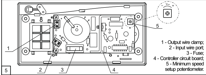
5 1 - Output wire clamp; 2 - Input wire port; 3 - Fuse; 4 - Controller circuit board; 5 - Minimum speed setup potentiometer.
